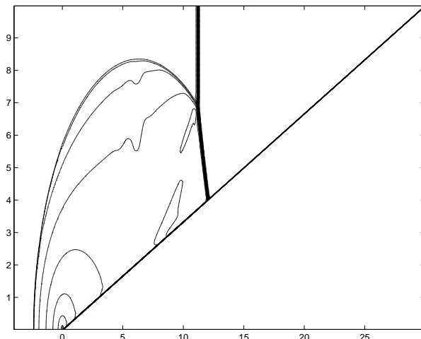
Figure 3: Density contours.
