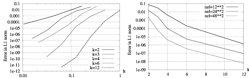
FIGURE 3.3. Convergence tests with spectral element approximation on smooth solution. Left: Galerkin solution; L^1 -norm of error versus mesh size h for various polynomial degrees k . Right: Entropy viscosity solution; L^1 -norm of error versus k for various mesh-sizes h .
