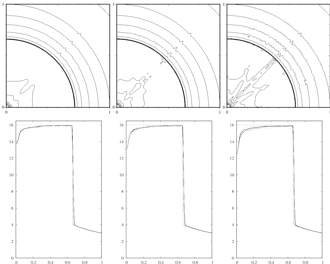
FIGURE 5.4. Noh test case at time t = 2 . Top: 23 density contours (from 2.5 to 4 with step 0.25 and from 14 to 17 with step 0.2). Bottom: Density profile versus radius along segments ( r \in (0, 1), \theta \in \{0, \frac{\pi}{8}, \frac{\pi}{4}, \frac{3\pi}{8}, \frac{\pi}{2}\} ). Left panels: \mathcal{P} = 1 . Center panel: \mathcal{P} = \frac{1}{2} . Right panel: \mathcal{P} = \frac{1}{4} .
