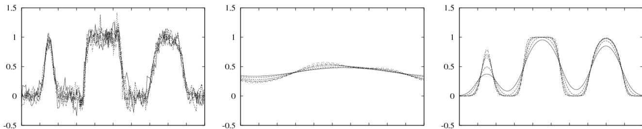
FIGURE 3.1. Long time integration, t = 100 , for polynomial degrees k = 2, \dots, 8 , #d.o.f.=200. Galerkin (left); Constant viscosity (center); Entropy viscosity (right).
