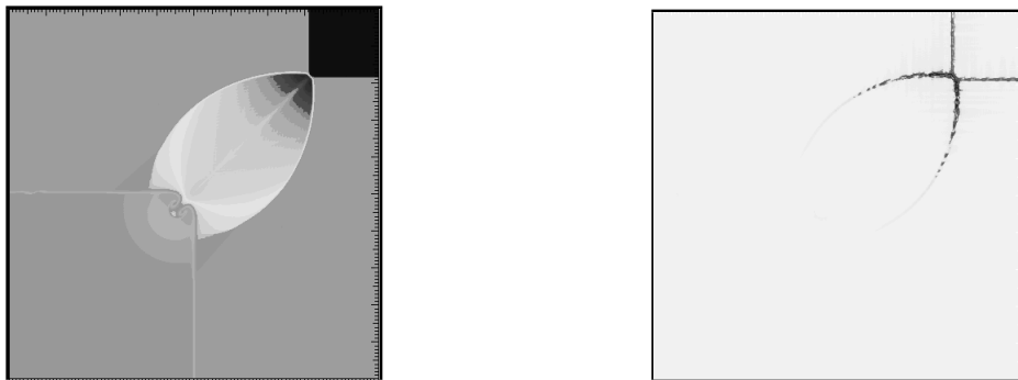
FIGURE 5.1. Riemann problem # 12, t = 0.2 , 400 \times 400 grid-points. Left: Density, 0.528 \leq \rho_h \leq 1.707 . Right: Viscosity, 0 \leq \mu_h < 3.410^{-3} .
