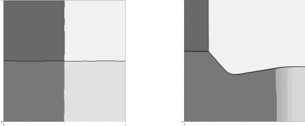
FIGURE 4.1. Burgers test case. Left: Initial data. Right: \mathbb{P}_1 approximation at t = 0.5 , 310^4 nodes
