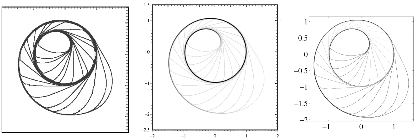
FIGURE 4.3. KPP rotating wave. Left: Entropy-viscosity with spectral elements, k = 4 on 96^2 elements. Center: entropy-viscosity \mathbb{P}_2 approximation, h = 0.0125 . Right: adaptive WENO5/Minmod 1 from [19] on Cartesian grid \Delta x = \Delta y = \frac{1}{100} .
