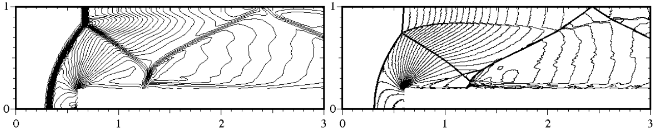
FIGURE 5.2. Mach 3 step, density, t = 4 , density, \mathbb{P}_1 approximation. Left: h = 0.25 , 4813 \mathbb{P}_1 nodes. Right: h = 0.003 , 893468 \mathbb{P}_1 nodes.
