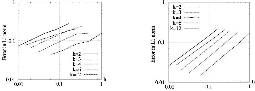
FIGURE 3.4. Convergence tests with the spectral element approximation on the non-smooth solution. L^1 -norm of the error vs. h for various k . Left: Galerkin. Right: Entropy viscosity.
