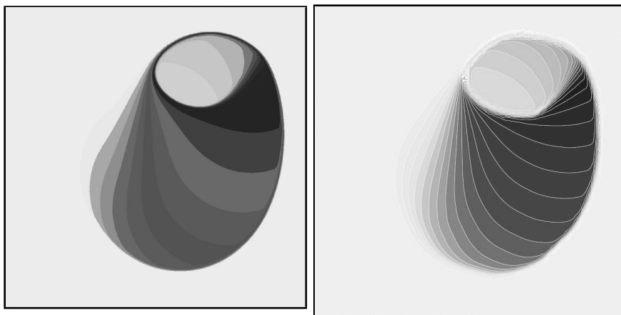
FIGURE 4.5. Buckley-Leverett test case. Left: \mathbb{P}_2 approximation, t = 0.5 , 6.710^4 nodes; Right \mathbb{P}_1 results using MAPR from [5] on uniform mesh with 10^4 nodes.
