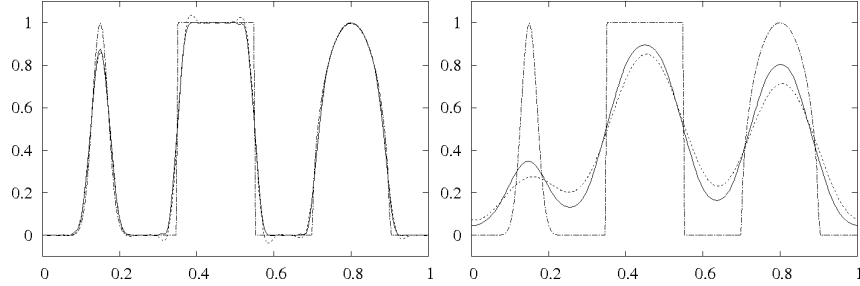
FIGURE 3.2. Dot-dashed line is the exact solution, solid line is the entropy viscosity solution, dashed line is the edge stabilized solution. Solutions at t = 1 (Left), solutions at t = 100 (Right).
