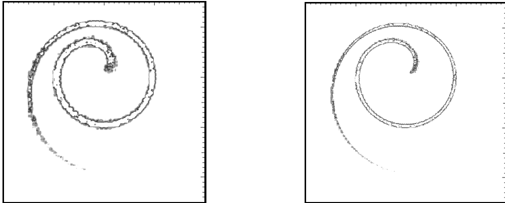
FIGURE 4.4. KPP rotating wave. Ratio \nu/\nu_{\max} for 48^2 and 96^2 elements. In both case the ratio saturates at \nu/\nu_{\max} = 1 , with \nu_{\max} \approx 0.016 and \nu_{\max} \approx 0.008 , respectively.
