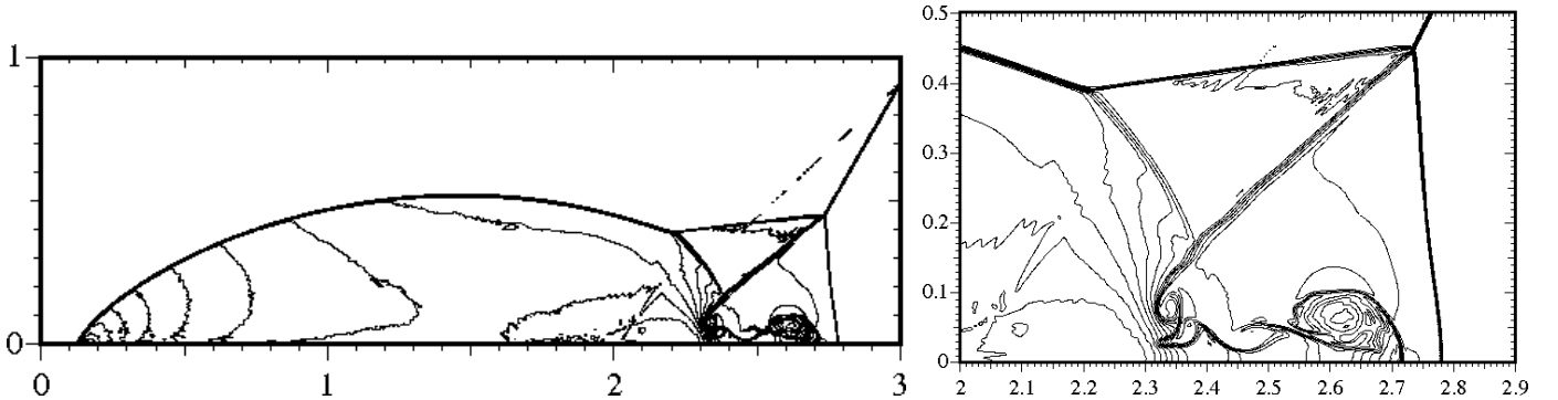
FIGURE 5.3. Double Mach reflection at t = 0.2 , M = 10 , density field, 453969 \mathbb{P}_1 nodes. Left: global view. Right: close up view in the region of three-shock interaction point.
