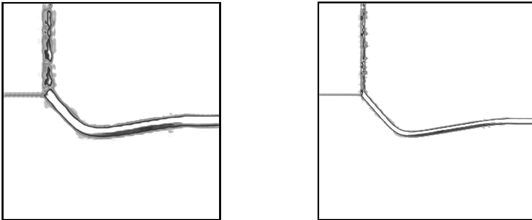
FIGURE 4.2. Entropy viscosity for the 96 \times 96 grid, 0 < \nu_h < 0.0050 (at left), and for the 192 \times 192 grid, 0 < \nu_h < 0.025 (at right).
