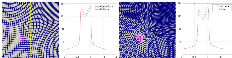
FIG. 5. Noh problem. From left to right: Zoom around the center of the nonuniform Q_1 mesh at T = 0.6 (notice the small displacement of the center); cross section along the line connecting the points (-1, -1) and (1, 1) for the Q_1 solutions on the uniform mesh and on the nonuniform mesh; zoom around the center of the nonuniform P_1 mesh at T = 0.6 ; cross section along the line connecting the points (-1, -1) and (1, 1) for the P_1 solutions on the uniform mesh and on the nonuniform mesh.
