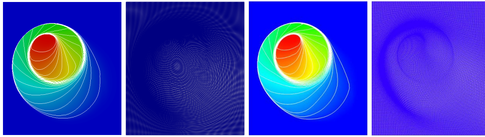
FIG. 2. KPP problem. Left: \mathbb{Q}_1 FEM with 25 contours. Center left: final \mathbb{Q}_1 mesh. Center right: \mathbb{P}_1 FEM with 25 contours. Right: final \mathbb{P}_1 mesh.
