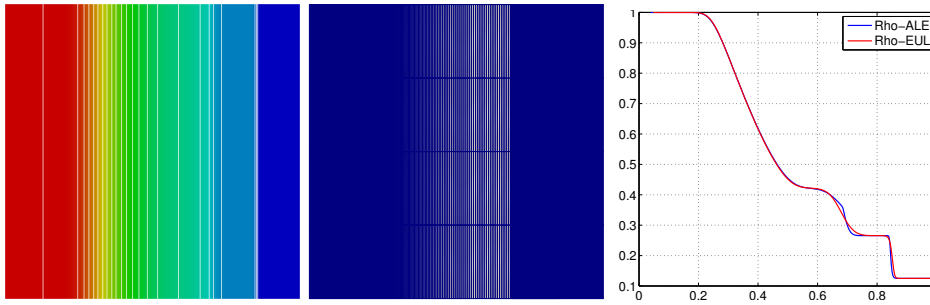
FIG. 3. Sod problem. Left: Q_1 FEM with 25 contours. Center: final Q_1 mesh.
