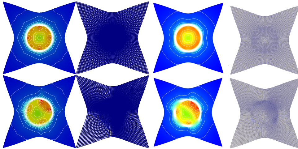
FIG. 4. Noh problem. Uniform meshes in top row, nonuniform meshes in bottom row. From left to right: density field with Q_1 approximation (25 contour lines); mesh with Q_1 approximation; density field with P_1 approximation (25 contour lines); mesh with P_1 approximation.
