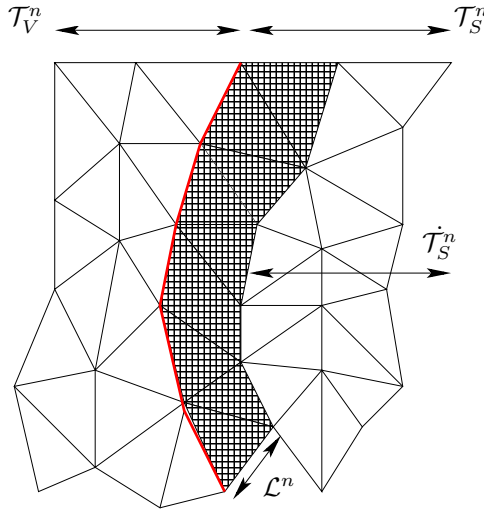
FIGURE 1. Schematic representation of the partition \mathcal{T} = \mathcal{T}_S^n \cup \mathcal{L}^n \cup \mathcal{T}_V^n .
