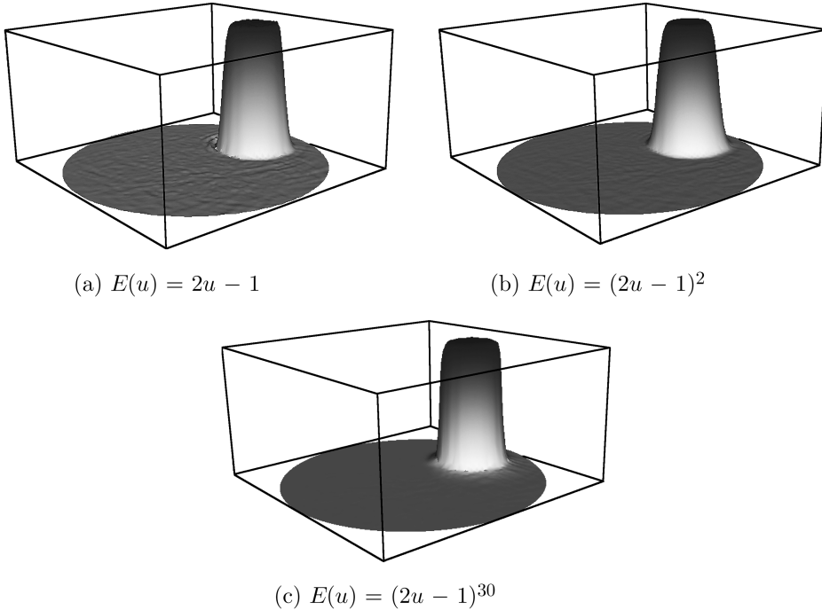
FIGURE 3. Tests on the linear transport equation with three different entropies.
