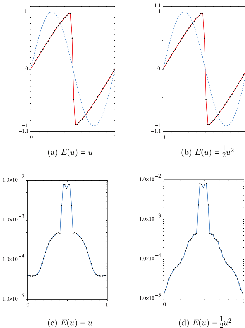
FIGURE 2. Burgers equation, \mathbb{P}_1 continuous finite elements, RK3, 50 elements.
