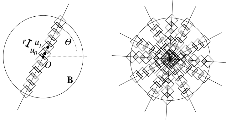
FIGURE 3. (a) A pin in the unit circle in \mathbb{R}^2 , with angle \theta . Here p = 1 , so that the \ell_p -balls are diamonds, and r is the \ell_2 -distance between consecutive centers (such as u_0 and u_1 ) of \ell_1 -balls. The petals are the shaded regions. (b) A pincushion consisting of several pins.
