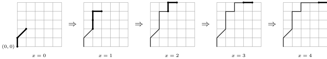
Figure 3: The steps of \phi that yield the corresponding Schröder path.
