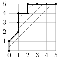
Figure 2: There are four tunnels in the Schröder path.
