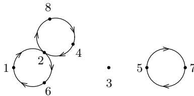
Figure 7: The cycle representation of the linked cycle \pi = (126)(284)(3)(57) .
