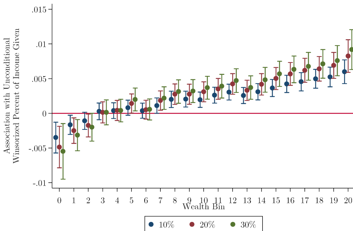
Figure A.4: Fixed Effects, Unconditional Winsorized Percent of Income Given, by Wealth
