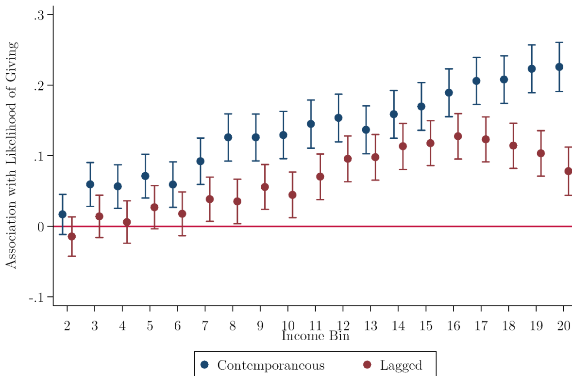
Figure A.10: OLS with Lags, Likelihood of Giving, by Income
