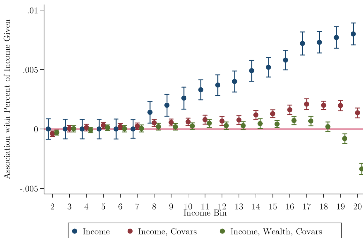
Figure A.5: Quantile Regressions (Median)
