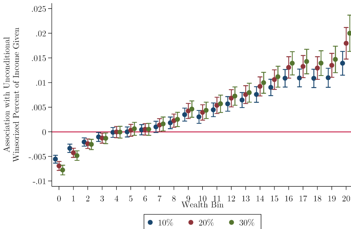
Figure A.2: OLS, Unconditional Winsorized Percent of Income Given, by Wealth
