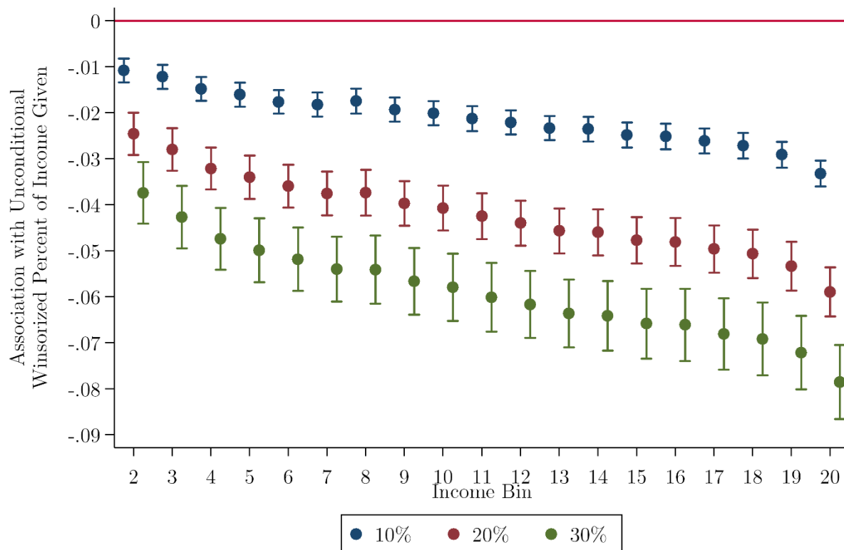
Figure A.3: Fixed Effects, Unconditional Winsorized Percent of Income Given, by Income
