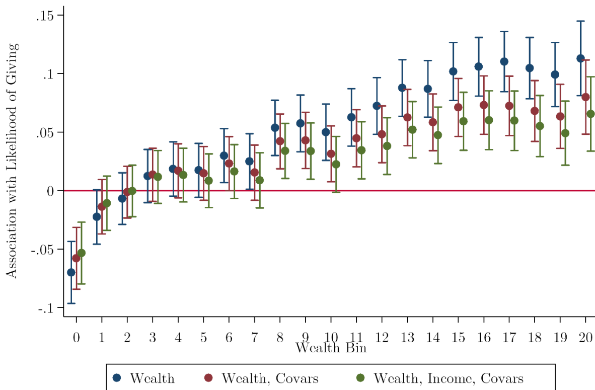
Figure 14: Fixed Effects, Likelihood of Giving, by Wealth
