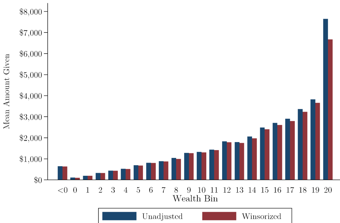
Figure 4: Amount Given, by Wealth
