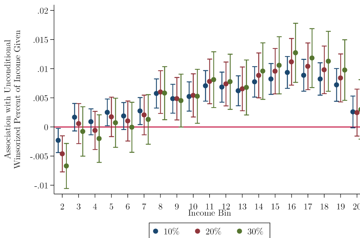
Figure A.1: OLS, Unconditional Winsorized Percent of Income Given, by Income
