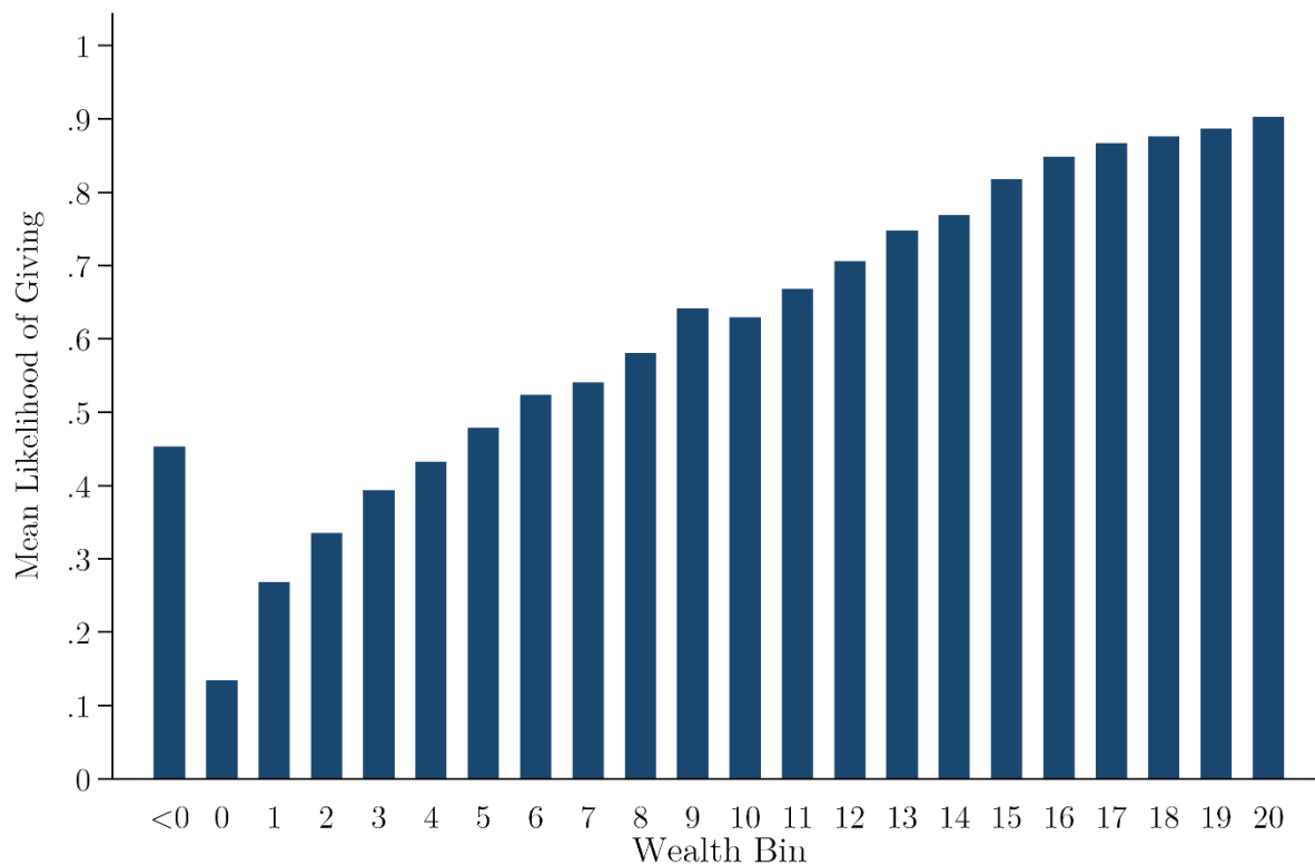
Figure 2: Likelihood of Giving, by Wealth
