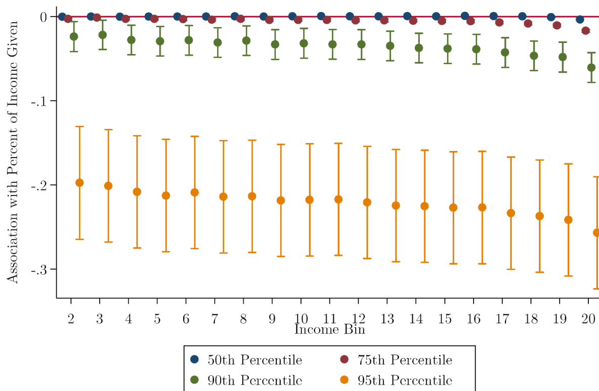
Figure A.7: Quantile Regressions
