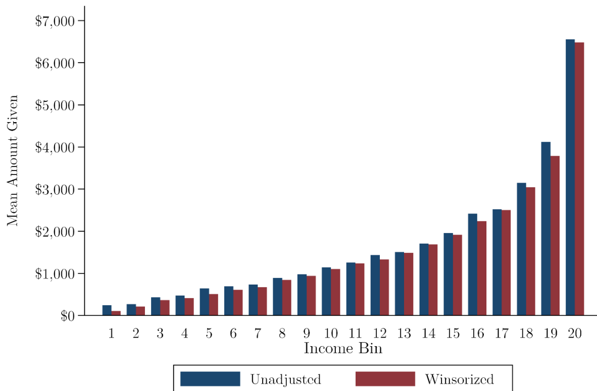
Figure 3: Amount Given, by Income
