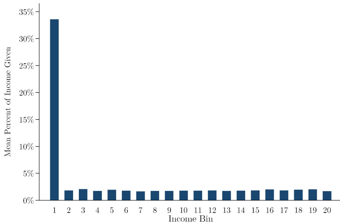
Figure 5: Percent of Income Given, by Income
