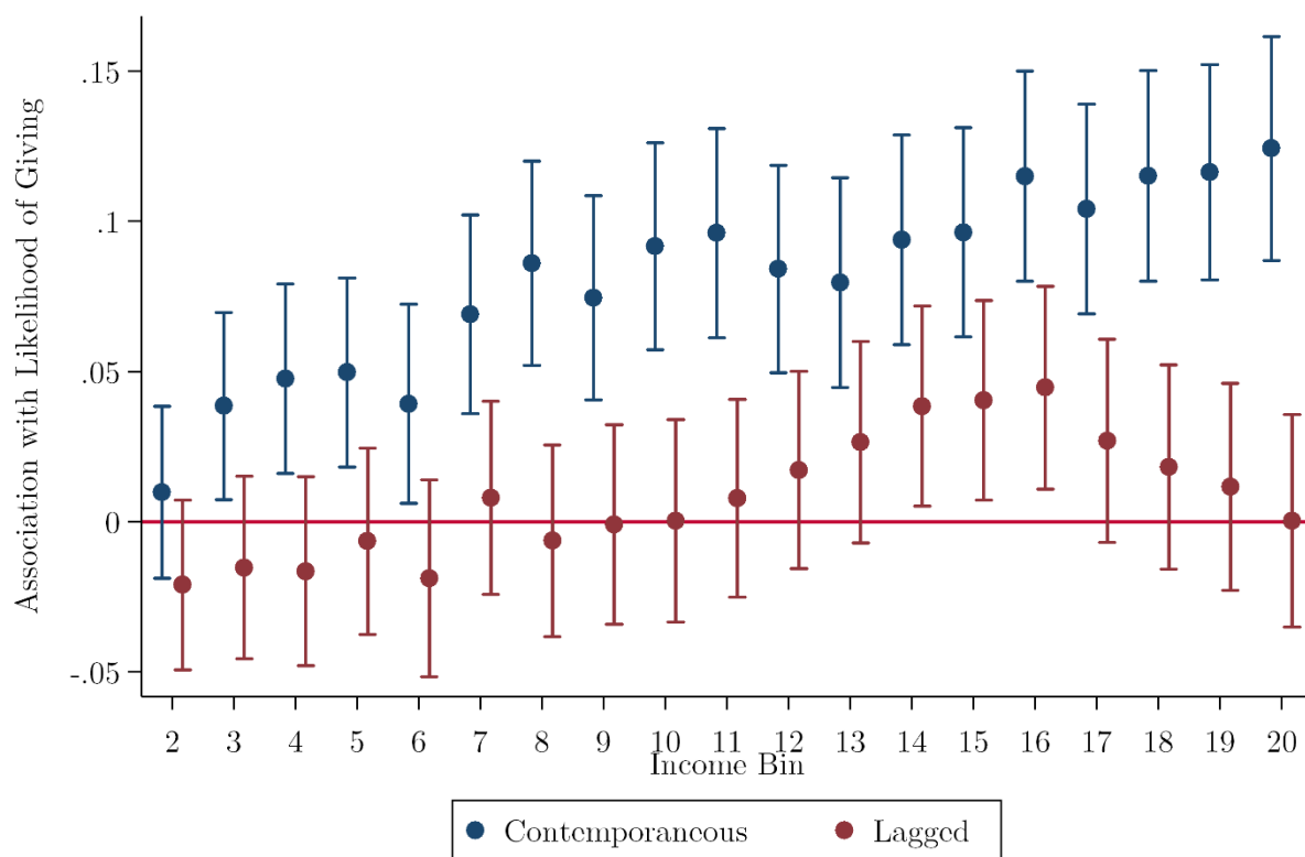
Figure A.11: FE with Lags, Likelihood of Giving, by Income
