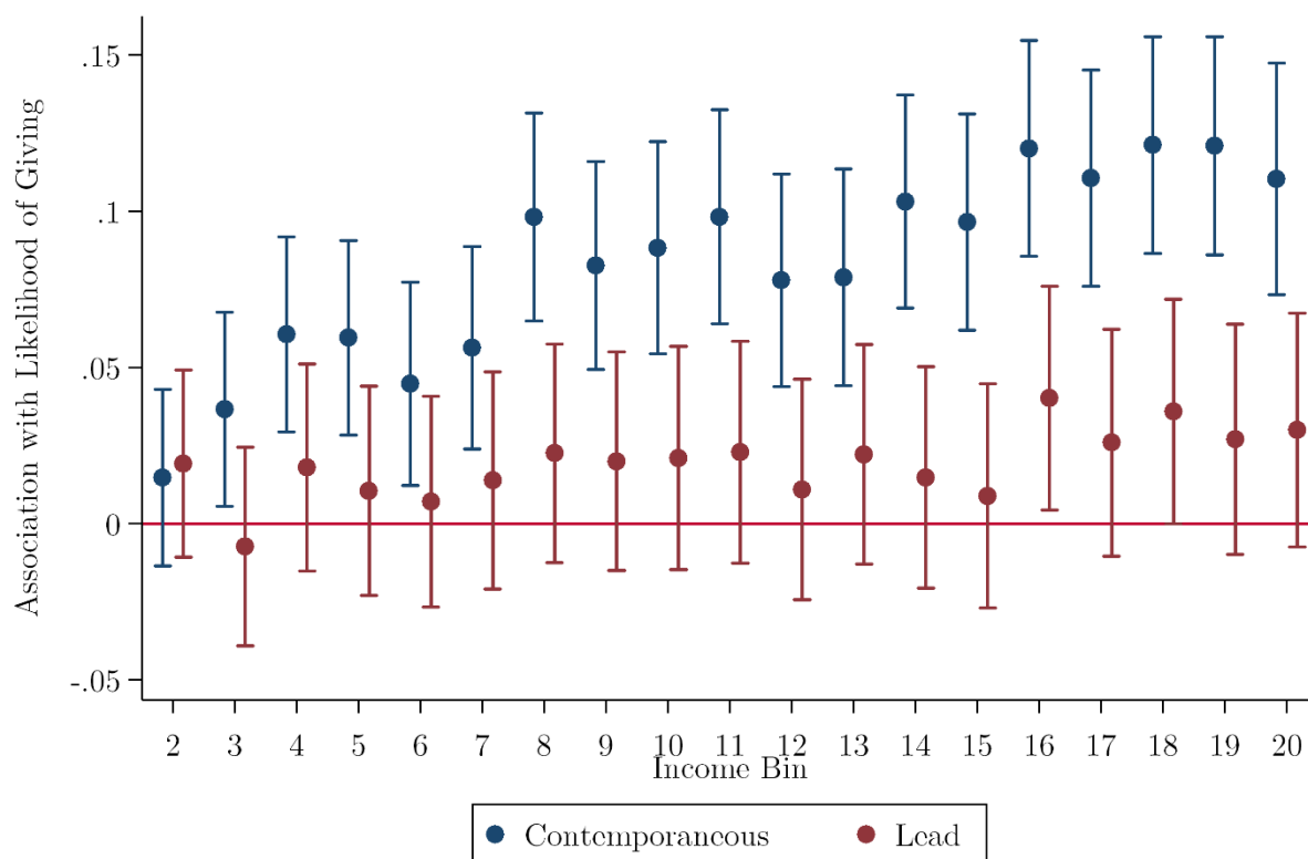
Figure A.13: FE with Leads, Likelihood of Giving, by Income
