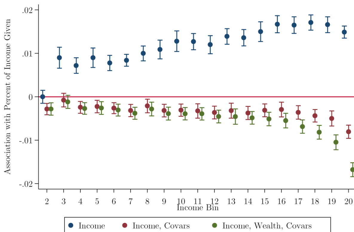
Figure A.6: Quantile Regressions (75 th Percentile)
