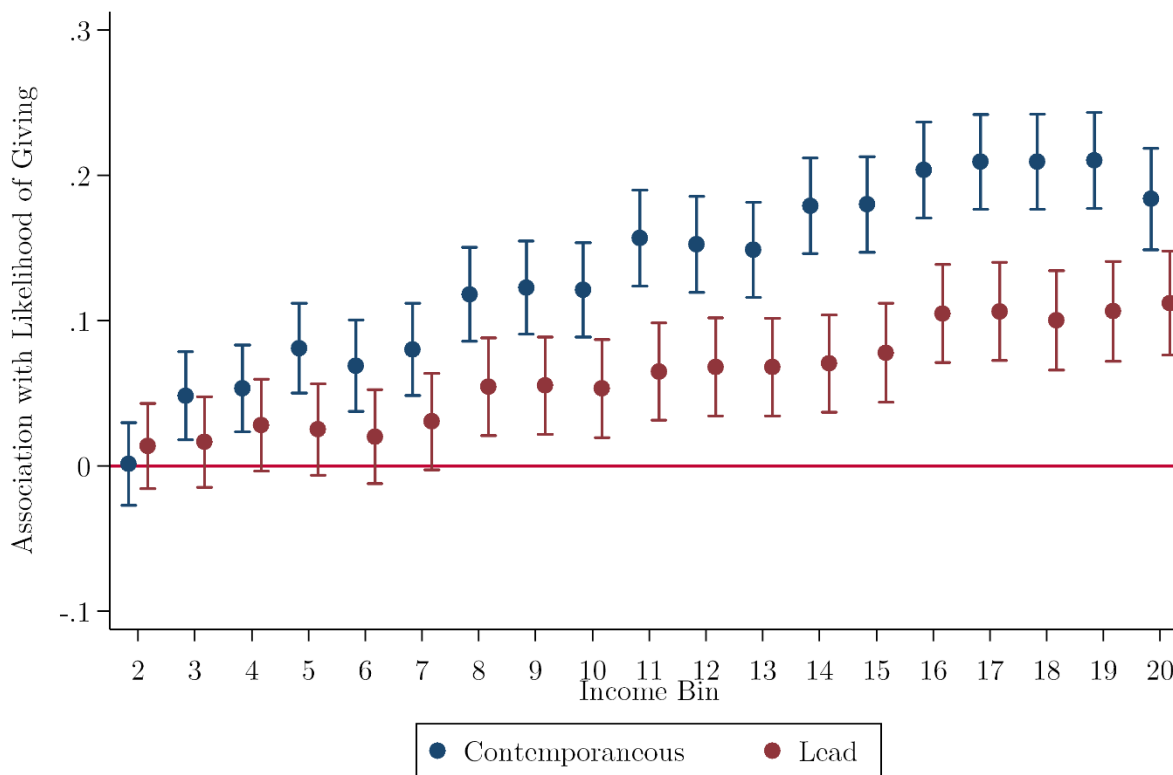
Figure A.12: OLS with Leads, Likelihood of Giving, by Income
