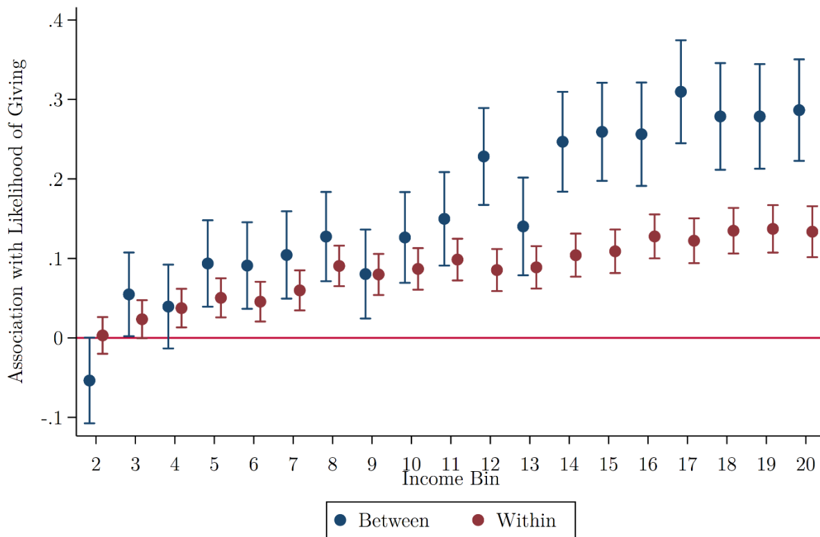
Figure A.8: Between vs Estimates, Likelihood of Giving, by Income
