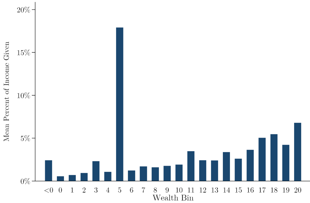
Figure 7: Percent of Income Given, by Wealth
