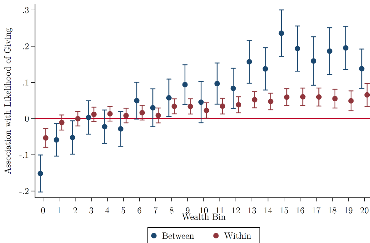
Figure A.9: Between vs Estimates, Likelihood of Giving, by Wealth
