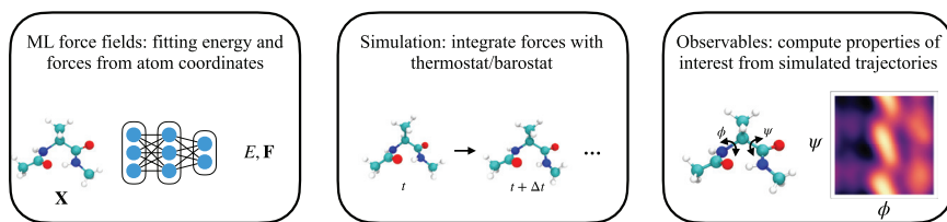
Figure 5.5: Simulating molecular dynamics with machine learning. To replace expensive quantum mechanical calculations, an ML force field is learned to predict energy and forces from atomic coordinates. With a learned force field, we can simulate MD by pairing it with an appropriate thermostat/barostat. From the simulated trajectories, properties of interest can be computed.
