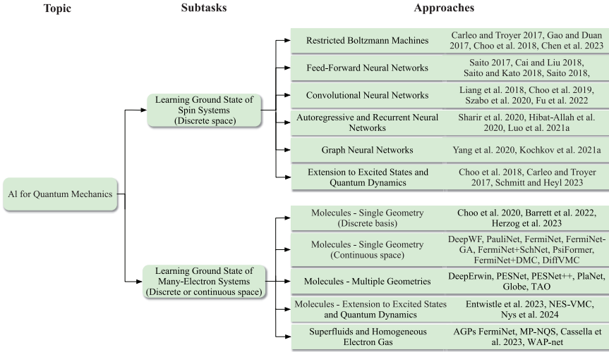
Figure 3.1: An overview of the tasks and methods in AI for quantum mechanics. In this section, we focus on two subtasks including learning ground states of spin systems and learning ground states of many-electron systems. The methods for learning ground states of spin systems are grouped in terms of the category of the network they use to represent the quantum state. Specifically, Carleo and Troyer (2017), Gao and Duan (2017), Choo et al. (2018), and Chen et al. (2023) use restricted Boltzmann machines. Cai and Liu (2018), and Saito and Kato (2018), Saito (2017 and 2018) use feed-forward neural networks. Liang et al. (2018), Choo et al. (2019), Szabó and Castelnovo (2020), and Fu et al. (2022a) use convolutional neural networks. Sharir et al. (2020), Hibat-Allah et al. (2020), and Luo et al. (2021a) use autoregressive and recurrent neural networks. Yang et al. (2020) and Kochkov et al. (2021a) use graph neural networks. For learning ground states of many-electron systems, one important application is molecules. One category of methods, including Choo et al. (2020), Barrett et al. (2022), and Herzog et al. (2023) aim to optimize single geometry of a molecule using discrete basis. DeepWF (Han et al. , 2019) PauliNet (Hermann et al. , 2020), FermiNet (Pfau et al. , 2020), FermiNet-GA (Lin et al. , 2023a), FermiNet+SchNet (Gerard et al. , 2022), PsiFormer (von Glehn et al. , 2023), FermiNet+DMC (Ren et al. , 2023; Wilson et al. , 2021), and DiffVMC (Zhang et al. , 2023b), aim to optimize single geometry of a molecule in continuous space. Another category of methods, including DeepErwin (Scherbela et al. , 2022), PESNet (Gao and Günnemann, 2021), PESNet++ & PlaNet (Gao and Günnemann, 2023b), Globe (Gao and Günnemann, 2023a), and TAO (Scherbela et al. , 2023), aim to optimize multiple geometries of the same molecule or even among different molecules simultaneously. Beyond molecules, AGPs FermiNet (Lou et al. , 2023) is developed for superfluids. MP-NQS (Pescia et al. , 2023), Cassella et al. (2023), and WAP-net (Wilson et al. , 2023) are developed for homogeneous electron gas. Beyond ground states, Choo et al. (2018) study excited states for spins and bosons. Entwistle et al. (2023) and Pfau et al. (2024) study excited states for molecules. Carleo and Troyer (2017) and Schmitt and Heyl (2020) study quantum dynamics for spin systems, and Nys et al. (2024) study quantum dynamics for molecules.
