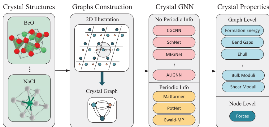
Figure 7.2: Pipeline of material representation learning. A crystalline material is transformed into a crystal graph representation, subsequently serving as the input for a crystal graph message passing neural network. Then the models are trained to accurately predict the desired properties of the crystal. Notably, a message passing process can be distinguished based on its incorporation of periodic information, such as lattice lengths or infinite potential summations. Networks without periodic information include models such as CGCNN (Xie and Grossman, 2018), SchNet (Schütt et al. , 2018), MEGNet (Chen et al. , 2019a), and ALIGNN (Choudhary and DeCost, 2021), among others. Conversely, networks that incorporate periodic information include Matformer (Yan et al. , 2022), PotNet (Lin et al. , 2023d), and Ewald-MP (Kosmala et al. , 2023). Additionally, the predicted output can be classified into graph-level properties, including formation energies and band gaps, or node-level properties, which include forces.
