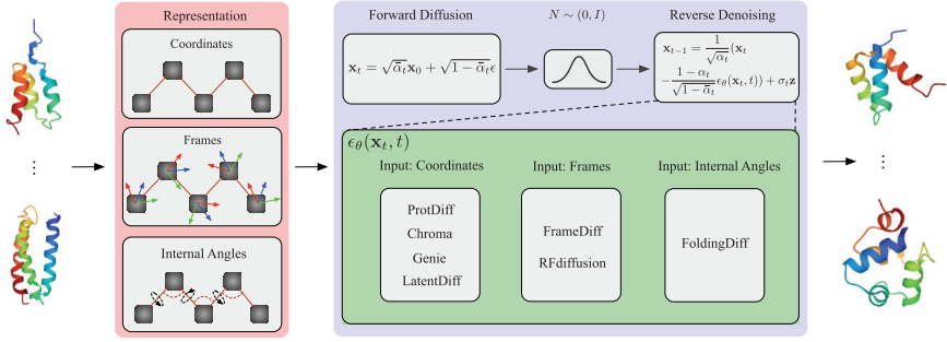
Figure 6.4: Pipeline of protein generation with diffusion models. The process begins by diffusing protein backbone structures to Gaussian noise, which is then denoised using a learned denoising network to generate novel protein structures. Protein backbones can be represented in various ways, such as coordinates, frames, or internal angles. Different methods have been proposed for each representation. For coordinates representation, methods include ProtDiff (Trippe et al. , 2022), Chroma (Ingraham et al. , 2022), LatentDiff (Fu et al. , 2023a) (coordinates are in the latent space), and Genie (Lin and AlQuraishi, 2023). For frames representation, methods include FrameDiff (Yim et al. , 2023a) and RFdiffusion (Watson et al. , 2022). For internal angles representation, the method is FoldingDiff (Wu et al. , 2022a).
