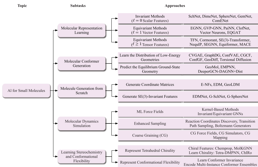
Figure 5.1: An overview of the tasks and methods in AI for small molecules. In this section, we consider five tasks, including molecular representation learning, molecular conformer generation, molecule generation from scratch, molecular dynamics simulation, and learning stereochemistry and conformational flexibility. In molecular representation learning, the \ell = 0 case corresponds to invariant methods, including SchNet (Schütt et al. , 2018), DimeNet (Gasteiger et al. , 2020), SphereNet (Liu et al. , 2022f), GemNet (Gasteiger et al. , 2021), and ComENet (Wang et al. , 2022g). The \ell = 1 case corresponds to equivariant methods with order-1 vector features \mathbf{v} \in \mathbb{R}^{d \times 3} , including EGNN (Satorras et al. , 2021a), GVP-GNN (Jing et al. , 2021), PaiNN (Schütt et al. , 2021), CiofNet (Du et al. , 2022), Vector Neurons (Deng et al. , 2021), and EQGAT (Le et al. , 2022). The \ell \geq 1 case corresponds to equivariant methods with order- \ell features \mathbf{h}^\ell \in \mathbb{R}^{d \times (2\ell+1)} , including TFN (Thomas et al. , 2018), 3d-steerable CNNs (Weiler et al. , 2018), Cormorant (Anderson et al. , 2019), SE(3)-Transformer (Fuchs et al. , 2020), NequIP (Batzner et al. , 2022), SEGNN (Brandstetter et al. , 2022a), Equiformer (Liao and Smidt, 2023), and MACE (Batatia et al. , 2022b). In molecular conformer generation, one category of methods aims to learn the distribution of low-energy geometries, including CVGAE (Mansimov et al. , 2019), GraphDG (Simm and Hernández-Lobato, 2019), ConfVAE (Xu et al. , 2021c), CGCF (Xu et al. , 2021a), ConfGf (Shi et al. , 2021), GeoDiff (Xu et al. , 2022a), and Torsional Diffusion (Jing et al. , 2022). Another category of methods aims to predict only the equilibrium ground-state geometry, including GeoMol (Ganea et al. , 2021), EMPNN (Xu et al. , 2023c) and DeeperGCN-DAGNN+Dist (Xu et al. , 2021d). In molecule generation from scratch, one category of method aims to directly generate coordinate matrices of 3D molecules, including E-NFs (Satorras et al. , 2021a), EDM (Hooeboom et al. , 2022), and GeoLDM (Xu et al. , 2023b). Another category of methods implicitly generates 3D atom positions from SE(3)-invariant features, including EDMNet (Hoffmann and Noé, 2019), G-SchNet (Gebauer et al. , 2019),
