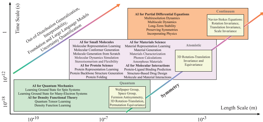
Figure 1.3: Spatial and temporal scale of scientific areas. We explore the intersection of AI and various scientific disciplines within a continuum of spatial and temporal scales. This framework accommodates a diverse range of areas and problems, unified by their distinct symmetries and shared technical challenges. Symmetries, inherent to the structure of natural science and governed by mathematical and physical laws, manifest in numerous patterns across various scientific fields. This cross-disciplinary perspective provides a fresh lens through which we can address and investigate complex scientific problems with AI methods.
