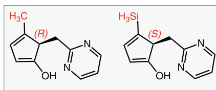
Figure 5.7: Global (R/S) chiral atom tags do not conserve local 3D geometric features. Small changes to the molecular graph, such as swapping a carbon atom for a silicon atom, can flip the handedness of a tetrahedral chiral centers (according to CIP rules) without affecting the 3D molecular geometry or chemical reactivity.
