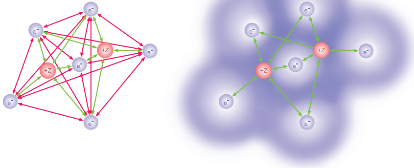
Figure 4.2: An illustration contrasting the interacting many-body perspective (left) with the DFT perspective within the Kohn-Sham framework (right) for modeling electronic structure in an atomistic system (e.g., molecules). Red spheres represent nuclei and blue spheres represent electrons. Red and green edges represent interactions between electron-electron pairs and electron-nucleus pairs (e.g., via Coulomb potential), respectively. The blue shading on the right represents the electron density. Left: In the interacting many-body view, the wavefunction of the system is defined w.r.t. the coordinates of all particles. Hence the interactions between all electron-electron and electron-nucleus pairs are explicitly considered, leading to an exponential growth of the dimension for many-body wavefunctions with the increasing number of electrons. Right: In the DFT Kohn-Sham picture, the electron-electron interactions are replaced by the interaction between each electron and the average effect of all other electrons, modeled with an electron density. Since such interactions are equivalent for different electrons, modeling the electronic wavefunction of the system effectively reduces to modeling multiple single-electron wavefunctions. The lighter shading around each electron illustrates the exclusion of the electron itself in the electron density to avoid the self-interaction.
