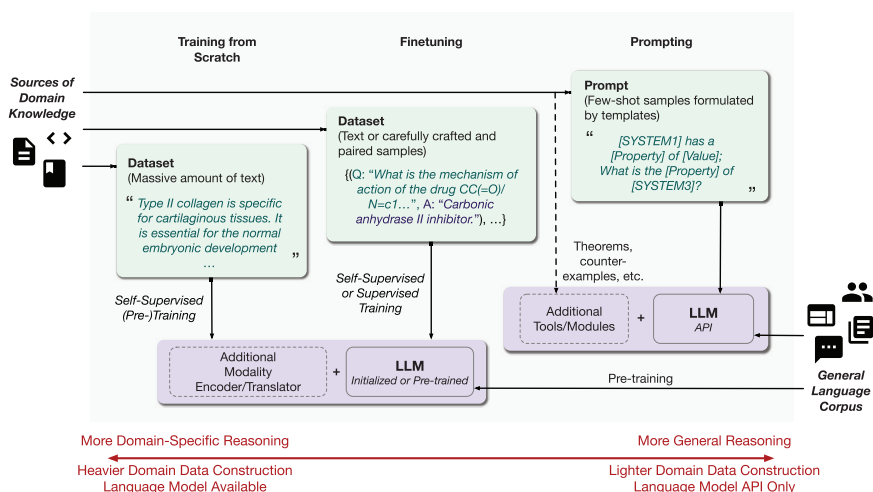
Figure 10.3: Three paradigms of adapting LLMs to science domains. One can construct datasets consisting of massive amounts of text from science domains and train LLMs from scratch in a self-supervised manner. The trained model can be used directly or further fine-tuned for specific tasks. Alternatively, one can fine-tune a pre-trained general-purpose LLM with less amount of text data, in a self-supervised manner, or paired samples, in a supervised manner, from science domains. In cases of proprietary LLMs with API access, one can adapt the model by prompting with carefully designed templates, where domain knowledge are provided as few-shot samples in the prompt or as explicit knowledge with additional tools or modules. Dataset examples are from Galactica (Taylor et al. , 2022) and ChEMBL (Liang et al. , 2023), respectively.
