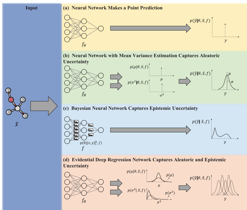
Figure 10.4: Schematic illustration of different uncertainty quantification methods on a molecular energy prediction task, with \hat{y} denoting the predicted energy of a given molecule. Note that (c) Bayesian Neural Network can be further combined with Mean Variance Estimation to capture both aleatoric and epistemic uncertainty.
