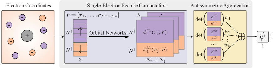
Figure 3.3: Pipeline of many-electron wavefunction computation with Slater determinants, illustrated for molecules. The input to the network is a set of 3D electron coordinates with N^\uparrow electrons with spin-up and N^\downarrow electrons with spin-down. The spin structure ( \uparrow or \downarrow ) as well as the positions of atomic nuclei are fixed. A neural network is used to produce k (N^\uparrow + N^\downarrow) -dimensional features vectors for each electron, which are then concatenated into k (N^\uparrow + N^\downarrow) \times (N^\uparrow + N^\downarrow) matrices. Finally, the determinants of these matrices are computed and a linear combination of them gives the final wavefunction value.
