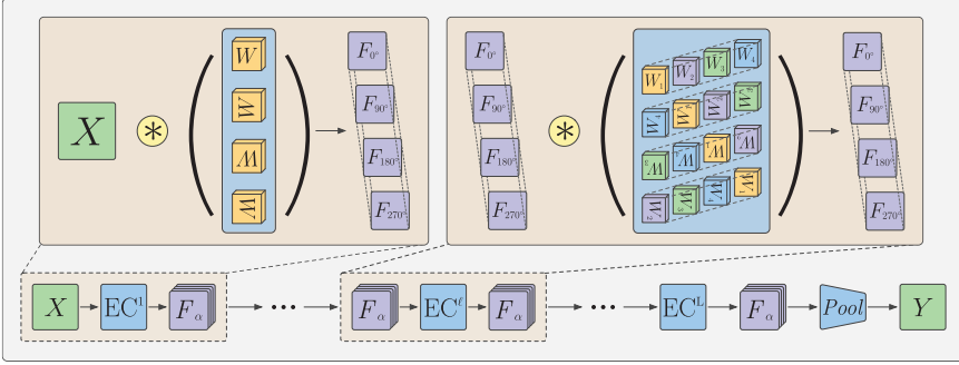
Figure 2.2: Illustration of equivariant convolutional neural networks as in G-CNNs (Cohen and Welling, 2016). The network passes input through an equivariant convolution layer (EC), resulting in a set of four output feature maps. If the input X is rotated by 90^\circ , 180^\circ , or 270^\circ , these feature maps will be rotated by \beta and their ordering permuted. Following this, L group convolution layers are applied, and a final pooling layer is added to account for the feature map permutations. This network is equivariant to rotations by 90^\circ , 180^\circ , or 270^\circ .
