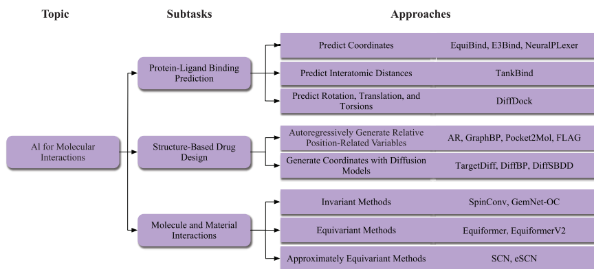
Figure 8.2: An overview of the tasks and methods in AI for molecular interactions. This section considers three tasks, including protein-ligand binding prediction, structure-based drug design, and energy, force, and position prediction for molecule-material pairs. In protein-ligand binding prediction, one category of methods, including EquiBind (Stärk et al. , 2022b), E3Bind (Zhang et al. , 2023c), and NeuralPLexer (Qiao et al. , 2023), aims to directly predict the 3D coordinates of ligands. In comparison, TankBind (Lu et al. , 2022b) predicts the interatomic distances between protein segments and ligands. Besides, DiffDock (Corso et al. , 2022) generates the rotation, translation, and torsion angles of seed conformers given by RDKit. In structure-based drug design, one category of methods, including AR (Luo et al. , 2021b), GraphBP (Liu et al. , 2022a), Pocket2Mol (Peng et al. , 2022), and FLAG (Zhang et al. , 2023d), aims to generate ligand atoms/fragments autoregressively by modeling their relative position-related variables. Another category of methods, including TargetDiff (Guan et al. , 2023), DiffBP (Lin et al. , 2022), and DiffSBDD (Schneuing et al. , 2022), considers generating 3D coordinates of all ligand atoms directly via diffusion models. In the prediction tasks for molecule-material pairs, the invariant methods are SpinConv (Shuaibi et al. , 2021) and GemNet-OC (Gasteiger et al. , 2022), and the equivariant methods include Equiformer (Liao and Smidt, 2023) and EquiformerV2 (Liao et al. , 2023). Besides, SCN (Zitnick et al. , 2022) and eSCN (Passaro and Zitnick, 2023) are approximately equivariant methods.
