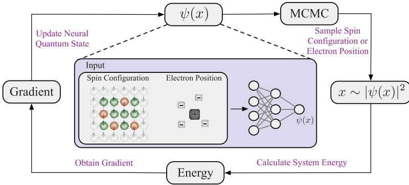
Figure 3.2: Pipeline of variational Monte Carlo (VMC). The neural quantum state takes as input a spin configuration or electron positions and outputs the wavefunction value. In VMC, spin configurations or electron positions are sampled using Markov chain Monte Carlo (MCMC) according to the probability distribution determined by the wavefunction. And then, energy is calculated from these samples, and the neural quantum state is updated by the gradient of the energy.
