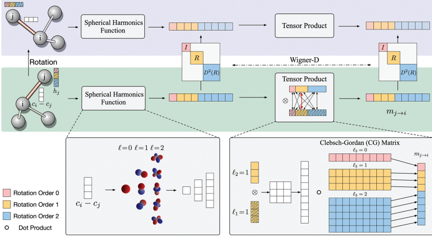
Figure 2.3: Illustrations of tensor product operations (Thomas et al. , 2018; Weiler et al. , 2018). Here we show how to compute a message m_{j \rightarrow i} from node j to node i , assuming the rotation orders are up to 2. Given the coordinates c_i and c_j of node i and node j in a 3D point cloud, their relational position c_i - c_j is first encoded into an SE(3) -equivariant feature vector using spherical harmonics functions. A tensor product is then performed between the computed feature vector and SE(3) -equivariant node features h_j of node j to compute the message m_{j \rightarrow i} . The resulting message m_{j \rightarrow i} is SE(3) -equivariant, rotating with the 3D point cloud via the corresponding Wigner-D matrix.
