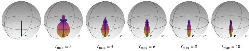
Figure 2.4: Illustration of spherical harmonics projection for a single unit vector. From left to right, a unit vector \mathbf{r} and its reconstruction from the spherical harmonics projection are plotted. A unit vector represents the Dirac delta on the unit sphere \mathbb{S}^2 , with a non-zero value only in the direction it points to. Spherical harmonics projection gives the spherical expansion of the Dirac delta on \mathbb{S}^2 as a linear combination of spherical harmonics. Since the spherical harmonics projection contains an infinite number of terms, in the figure reconstructions are only considered within finite truncated terms for simplicity. Specifically, each sub-figure above from left to right corresponds to a finite subset of terms from the spherical harmonics projection, for \ell_{\max} = 2 , \ell_{\max} = 4 , \ell_{\max} = 6 , \ell_{\max} = 8 , and \ell_{\max} = 10 , respectively. To visualize a function on the sphere clearly, the reconstruction is plotted as a 3D blob around the vector \mathbf{r} where the distance to the origin represents the function magnitude on the sphere along that direction. Additionally, the maximum amplitude in the reconstruction is scaled to one for visualization. As illustrated by the above sub-figures, increasing the value of \ell_{\max} leads to a progressively thinner 3D blob, approximating the Dirac delta on the sphere. This example is adapted from lecture notes by Tess Smidt with permission.
