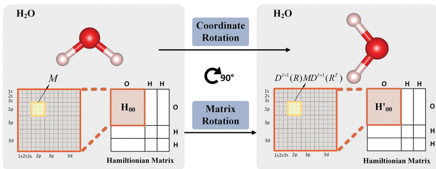
Figure 4.4: The equivariance of Hamiltonian matrix \mathbf{H} . When the coordinates of the molecule are rotated using a rotation matrix \mathbf{R} , the corresponding Hamiltonian matrix is rotated accordingly. Specifically, the Hamiltonian block B represents the orbital interaction between the oxygen 2p orbitals, and it is rotated to D^{\ell=1}(\mathbf{R}) B D^{\ell=1}(\mathbf{R}^T) using Wigner D-matrix D^\ell(\mathbf{R}) .
