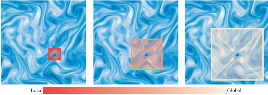
Figure 9.2: Multi-scale dynamics. Many systems exhibit dynamics consisting of interacting components with sizes ranging from local to global scales. A primary example is turbulent flows, which possess a hierarchy of eddies that decay down to the smallest scale, referred to as the Kolmogorov scale (Pope, 2000). Constructing machine learning models with multi-scale processing mechanisms is therefore key for high-fidelity simulation. These mechanisms aggregate information on each scale to update the latent representation at each mesh point. Here, we visualize a mechanism that performs aggregation and updates on each scale sequentially, as considered by Stachenfeld et al. (2021) and Gupta and Brandstetter (2023), however, mechanisms such as those proposed by Li et al. (2021e) and Lam et al. (2022) act in parallel.
