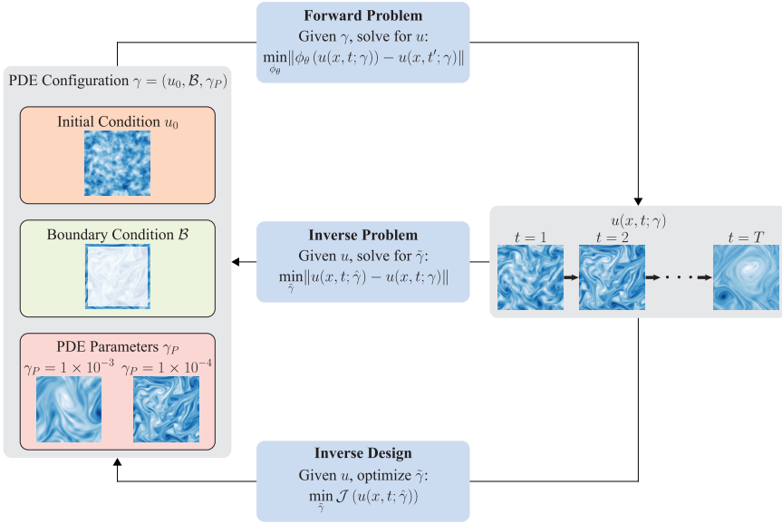
Figure 9.4: Illustration and comparison of forward problems, inverse problems, and inverse design. The solution to a PDE u(x, t; \gamma) sampled on grid points (x, t) discretizing space-time is induced by the PDE configuration \gamma = (u_0, \mathcal{B}, \gamma_P) describing the initial conditions u_0 , boundary conditions \mathcal{B} , and PDE parameters \gamma_P . In forward problems, the task is to learn the mapping from the solution induced by a particular choice of \gamma at earlier time steps t to the solution at later time steps t' > t using the forecasting model \phi_\theta . Conversely, inverse problems consider the task of identifying a subset of the PDE configuration \hat{\gamma} \subset \gamma , such as the initial conditions u_0 , that generated the observed rollout data. The data is assumed to have originated from a forward model u(x, t; \gamma) , and the estimated configuration \hat{\gamma} is optimized by minimizing the discrepancy between u(x, t; \hat{\gamma}) and the observed data u(x, t; \gamma) , where \hat{\gamma} denotes the union of the estimated components of the configuration \hat{\gamma} with the known components. Lastly, inverse design involves identifying \hat{\gamma} \subset \gamma such that the resulting rollout u(x, t; \hat{\gamma}) optimizes some criterion \mathcal{J} , such as identifying the shape of an airplane wing that minimizes drag.
