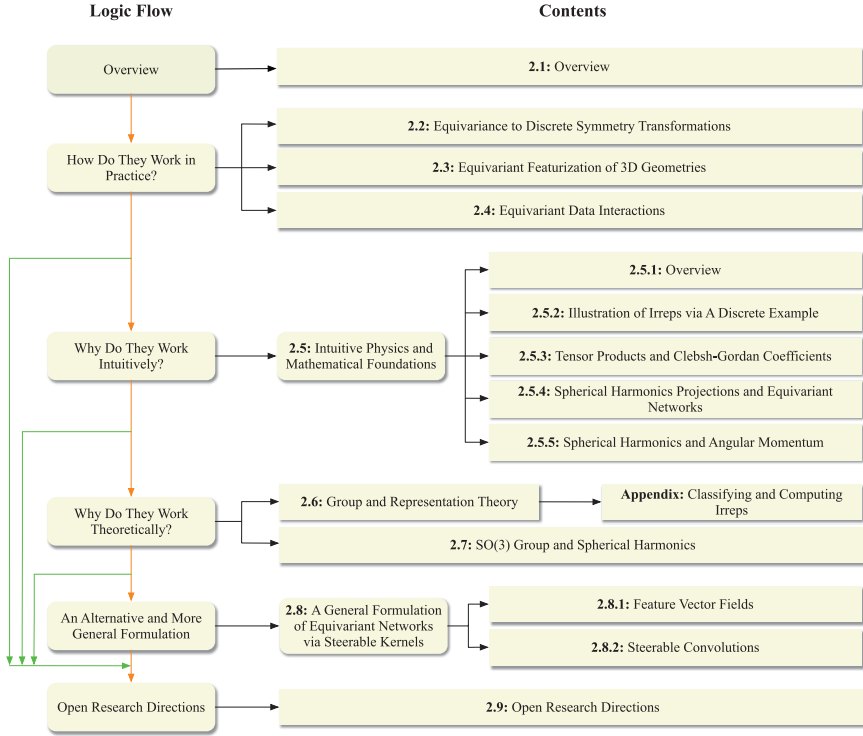
Figure 2.1: The overall logic flow and the associated subsections for Section 2. Note the arrows in the logic flow show the dependencies among different subsections, and especially, the green skip connections indicate that some subsections can be skipped. The black arrows show the associations between the logic flow and the subsections, as well as the relationships between each subsection and its child sections. Note the purpose of this figure is for readers to quickly navigate to certain contents based on background and interest, e.g., certain readers may skip the subsections associated with “Why Do They Work Theoretically?”.
