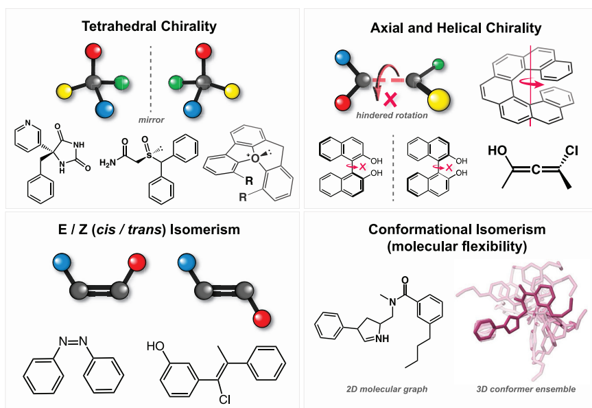
Figure 5.6: Stereochemistry is an important yet often overlooked aspect of molecular identity that describes the differing orientations or arrangements of atoms in 3D space for molecules which share a common 2D graph topology. Stereoisomerism can be caused by a variety of local structural characteristics; shown here are common forms of stereochemistry that are particularly relevant for medicinal chemistry, chemical catalysis, and organic chemistry. Tetrahedral chirality (or point chirality) describes the differing orientations of four non-equivalent chemical groups around a stereogenic center. Tetrahedral chiral centers are inverted upon reflection, and hence induce enantiomerism. Tetrahedral chirality is often associated with carbon atoms, but can arise elsewhere, such as in sulfinyl or oxonium compounds. Axial chirality is caused by the (non-planar) orientations of four chemical substituents around a chiral axis. Axial chirality is found in allenes due to the propeller-like arrangement of adjoining double ( \pi ) bonds, and commonly in atropisomers, where bulky substituents restrict rotation about a single ( \sigma ) bond. Helical chirality is also a form of axial chirality, although its structural origin is different. Like tetrahedral chirality, axial chirality leads to enantiomerism. E/Z isomerism is caused by the differing cis or trans configurations of (planar) double bonds. Unlike tetrahedral or axial chirality, E/Z isomerism does not produce pairs of enantiomers. These forms of stereochemistry yield stereoisomers that typically cannot be interconverted on practical timescales without undergoing chemical reactions. Any given stereoisomer can also have a distribution of structurally-distinct but rapidly-interconverting conformational isomers, or conformers , owing to the molecule's 3D flexibility. Observable molecular properties are often related to thermodynamic averages over the entire conformer ensemble.
