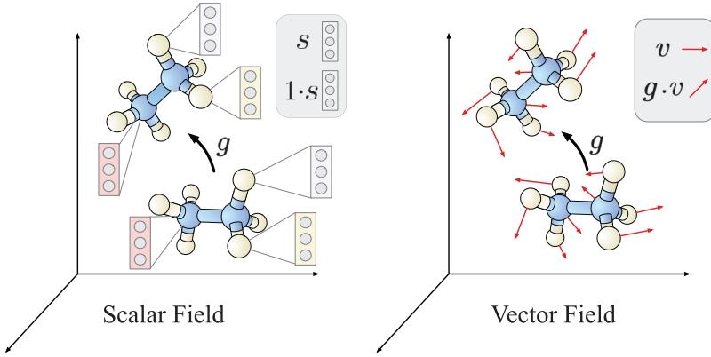
Figure 2.5: Scalar and vector fields as simple examples of feature vector fields. Affine groups act on such fields by (1) moving features across space (black arrow), and (2) transforming the features themselves via some group representation \rho . For the trivial representation \rho(g) = 1 , this explains scalar fields, while \rho(g) = g describes vector fields. All of the feature spaces in the example above correspond to some choice of G -representation, e.g., Wigner-D matrices \rho = D^\ell for tensor field networks and G = SO(3) . Steerable CNNs are built from layers which map in an equivariant way between feature fields, for instance from scalar to vector fields or vice versa. Linear equivariant maps are necessarily convolutions, however, with additionally symmetry constrained “steerable kernels”. This figure is adapted from Weiler and Cesa (2019) with permission.
