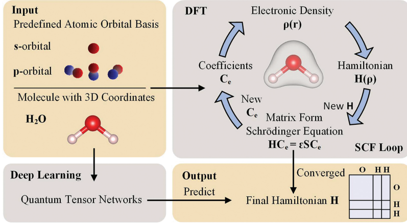
Figure 4.3: The pipeline of the DFT calculations and deep learning methods to obtain the Hamiltonian matrix. The DFT calculation uses the predefined atomic orbital basis associated with the molecule and its coordinates to optimize Hamiltonian matrix H(\rho) iteratively within the SCF loop until it reaches convergence towards the total energy minimum/minima. In contrast, deep learning method uses the proposed quantum tensor networks to directly predict the final Hamiltonian matrix, taking atomic types and coordinates as inputs. This eliminates the iterative optimization, thereby accelerating the DFT calculations.
