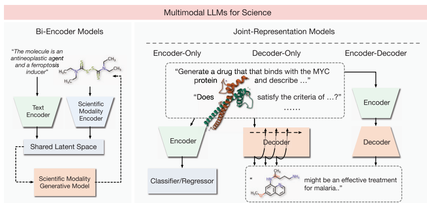
Figure 10.2: High-level architectures for multimodal scientific NLP. Molecule-language multimodality is used as a source for examples. The dotted lines in the bi-encoder diagram indicate the possible extension to a generative framework. Example inputs and outputs are shown with “code-switched” modalities (i.e., they are integrated into a single sequence). Encoders are used to generate an output representation which can be used for retrieval, classification, and regression, among other tasks. Decoder models are generally used for generative modeling applications. In some cases, non-LLM components can be used (such as for the decoder in an encoder-decoder model). We note that the extension of general-purpose LLMs via tools is another approach not shown in this figure.
