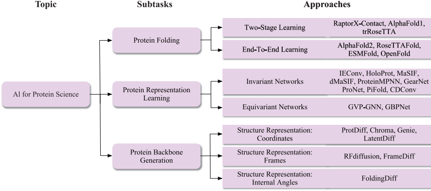
Figure 6.1: An overview of the tasks and methods in AI for protein science. In this section, we focus on three subtasks, including protein folding, protein representation learning, and protein backbone generation. The methods for protein folding can be categorized into two classes, before and after AlphaFold2 (Jumper et al. , 2021): (1) two-stage learning: RaptorX-Contact (Wang et al. , 2017b), AlphaFold1 (Senior et al. , 2020), trRoseTTA (Du et al. , 2021), (2) end-to-end learning: AlphaFold2 (Jumper et al. , 2021), RoseTTAFold (Baek et al. , 2021), ESMFold (Lin et al. , 2023e), OpenFold (Ahdritz et al. , 2022). The methods for protein representation learning are grouped into the invariant networks, including IEConv (Hermosilla et al. , 2021), HoloProt (Somnath et al. , 2021), MaSIF (Gainza et al. , 2020; Gainza et al. , 2023), dMaSIF (Sverrisson et al. , 2021), ProteinMPNN (Dauparas et al. , 2022), GearNet (Zhang et al. , 2023e), ProNet (Wang et al. , 2023a), PiFold (Gao et al. , 2023), and CDCConv (Fan et al. , 2023), and equivariant networks, including GVP-GNN (Jing et al. , 2021) and GBPNet (Aykent and Xia, 2022). For protein backbone generation, the methods are grouped in terms of structure representations they use. Specifically, ProtDiff (Wu et al. , 2022a), Chroma (Ingraham et al. , 2022), LatentDiff (Fu et al. , 2023a), and Genie (Lin and AlQuraishi, 2023) use 3D Euclidean coordinates as the structure representation for protein backbone structure, while RFdiffusion (Watson et al. , 2022) and FrameDiff (Yim et al. , 2023a) use frame representations. Besides, FoldingDiff (Wu et al. , 2022a) uses internal angles to represent protein backbone structures.
