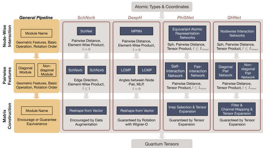
Figure 4.5: An overview of quantum tensor networks and methods in AI for density functional theory. Quantum tensor networks take the atomic types and coordinates of a given molecule as input and output the predicted quantum tensor, such as the Hamiltonian matrix. Typically, quantum tensor networks consist of three sequential modules: the node-wise interaction module, pairwise feature building module, and matrix construction module. The node-wise interaction module updates the node features based on neighboring nodes within a cutoff distance. The pairwise feature module creates features to describe the relationship between atom pairs, with a diagonal module for pairs of a single atom and a non-diagonal module for pairs of two atoms. Pairwise features are then used to construct target matrices for node pairs, which are assembled to output the quantum tensor for the entire molecule. In node-wise interaction and pairwise feature modules, existing methods use different geometric features, basic operations, and rotation orders in their designs. Note that Sph denotes the spherical harmonics of edge direction. In the matrix construction module, the equivariance of the constructed matrix is either encouraged or guaranteed through various techniques. This figure provides module names and essential information about each module for existing methods, including SchNorb (Schütt et al. , 2019), DeepH (Li et al. , 2022a), PhiSNet (Unke et al. , 2021c), and QHNet (Yu et al. , 2023b).
