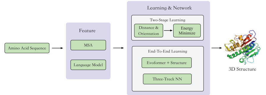
Figure 6.2: Summarization of the protein folding algorithms. Existing methods, including RaptorX-Contact (Wang et al. , 2017b), AlphaFold1 (Senior et al. , 2020), trRoseTTA (Du et al. , 2021), AlphaFold2 (Jumper et al. , 2021), RoseTTAFold (Baek et al. , 2021), AlphaFold-Multimer (Evans et al. , 2021), ESMFold (Lin et al. , 2023e), and OpenFold (Ahdritz et al. , 2022), follow this pipeline and their respective modules are summarized in Table 6.1.
