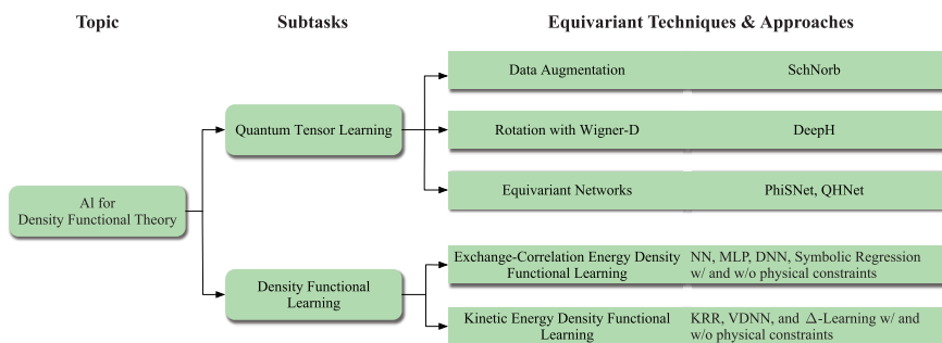
Figure 4.1: An overview of tasks and methods in AI for density functional theory (DFT). In the quantum tensor learning subtask, invariant quantum tensor networks include SchNorb (Schütt et al. , 2019) and DeepH (Li et al. , 2022a). SchNorb encourages the equivariance by training with data augmentation and DeepH guarantees the equivariance by rotation with Wigner D-matrix. Meanwhile, equivariant quantum tensor networks, including PhiSNet (Unke et al. , 2021c) and QHNet (Yu et al. , 2023b), intrinsically consider the equivariance of matrix by tensor product and tensor expansion. Another subtask is density functional learning, primarily focused on approximating exchange-correlation (XC) energy and kinetic energy. Several machine learning approaches have been employed for approximating exchange-correlation energy density functionals. These include neural network (NN) (Tozer et al. , 1996; Dick and Fernandez-Serra, 2019, 2020; Ryabov et al. , 2020; Lei and Medford, 2019; Gedeon et al. , 2021), multiple layer perceptron (MLP) (Nagai et al. , 2020), deep neural network (DNN) (Kirkpatrick et al. , 2021; Pokharel et al. , 2022), and symbolic regression (Ma et al. , 2022), implemented both with and without physical constraints. In terms of approximating kinetic energy density functionals, approaches such as kernel ridge regression (KRR) (Snyder et al. , 2012, 2015), voxel deep neural network (VDNN) (Ryczko et al. , 2022b), and \Delta -Learning (Ramakrishnan et al. , 2015) have been used, again both with and without the inclusion of physical constraints. Alternatively, Brockherde et al. (2017) aims to learn Hohenberg-Kohn map between external potential and electron density using KRR, thereby bypassing the Kohn-Sham equation.
