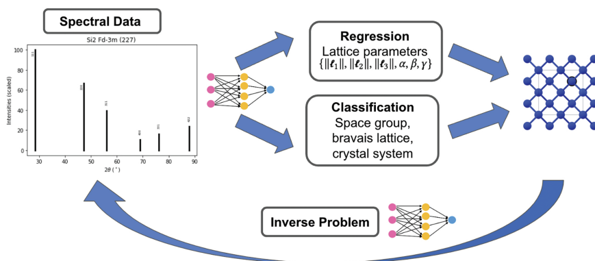
Figure 7.3: Potential applications of ML in materials characterization methods. Given spectral data, ML can be used for crystal structure prediction. This could entail a regression task (predicting the lattice parameters or atomic positions) or a classification task (predicting space group, bravais lattice, or crystal system). In the inverse task, ML is used to reconstruct diffraction spectra given the crystal structure.
