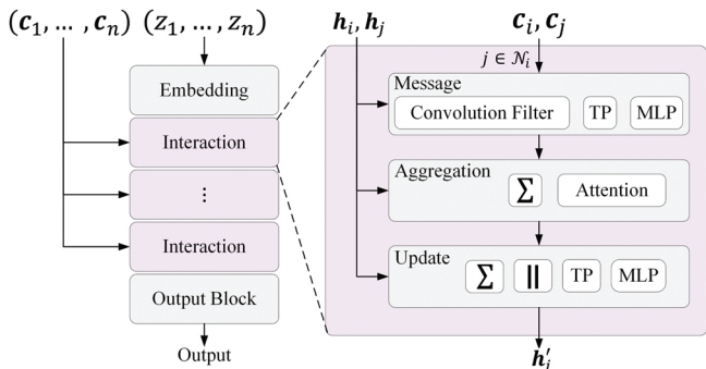
Figure 5.4: A general architecture of higher order equivariant models. Each model consists of several interaction blocks which perform pairwise message passing between atoms. Here, \Sigma denotes summation, \parallel denotes feature concatenation, TP refers to the Tensor Product of feature vectors, and MLP refers to multilayer perceptrons. The specific operations used in each Message, Aggregation, and Update blocks differ between models, but existing methods such as TFN (Thomas et al. , 2018), NequIP (Batzner et al. , 2022), SE(3) -Transformer (Fuchs et al. , 2020), Equiformer (Liao and Smidt, 2023), Cormorant (Anderson et al. , 2019), and SEGNN (Brandstetter et al. , 2022a) all fall under this framework.
