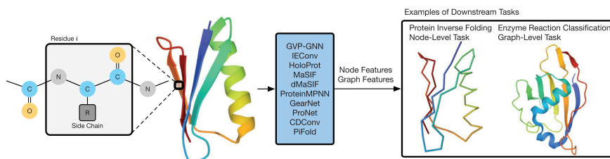
Figure 6.3: Illustrations of protein structures, representation learning methods, and examples of downstream tasks. Proteins consist of one or more amino acid chains. When two or more amino acids bond to form a peptide, water molecules are removed, and the remaining part of each amino acid is called an amino acid residue. The left part of the figure shows the detailed structure of a residue. In the middle, we list existing protein representation learning methods, including GVP-GNN (Jing et al. , 2021), IEConv (Hermosilla et al. , 2021), HoloProt (Somnath et al. , 2021), MaSIF (Gainza et al. , 2020; Gainza et al. , 2023), dMaSIF (Sverrisson et al. , 2021), ProteinMPNN (Dauparas et al. , 2022), GearNet (Zhang et al. , 2023e), ProNet (Wang et al. , 2023a), CDCConv (Fan et al. , 2023), and PiFold (Gao et al. , 2023). Different downstream tasks are shown in the right, including node-level tasks such as protein inverse folding (Ingraham et al. , 2019) and graph-level tasks such as enzyme reaction prediction (Hermosilla et al. , 2021).
