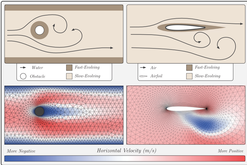
Figure 9.3: Multi-resolution dynamics, data from Pfaff et al. (2021). Systems with localized regions of fast-evolving dynamics, such as fluid flow around a cylinder (left) or air flow around an airfoil (right), require high-resolution discretizations in these regions for dynamics to be stably resolved. Irregular discretizations of the domain can manage this cost by allocating high resolution in regions of high gradient and coarse resolution elsewhere. However, since irregularly discretized functions cannot be modeled by architectures such as CNNs, there has been a call for GNNs for simulating dynamics (Pfaff et al. , 2021). Furthermore, the location in space of these high gradient regions can shift as the system evolves, thus requiring the discretization to dynamically adapt. While traditional re-meshing algorithms can be expensive, Pfaff et al. (2021) and Wu et al. (2022c) propose learned alternatives for adaptive mesh refinement that reduce this cost.
